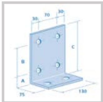
Purlin Cleat
